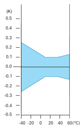
Temperature accuracy
