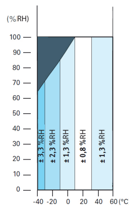
Humidity accuracy
